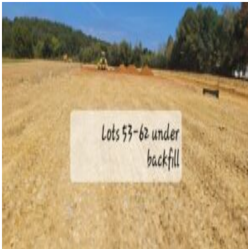
Picture depicting lots#53-62 backfilled and tested and have pretty good compaction
